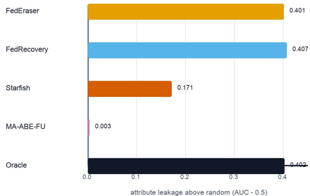
b Residual semantic-policy exposure
