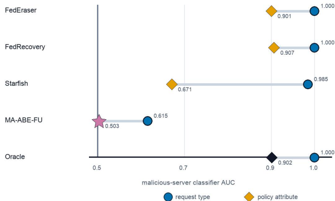
a Request-type and policy-attribute leakage
